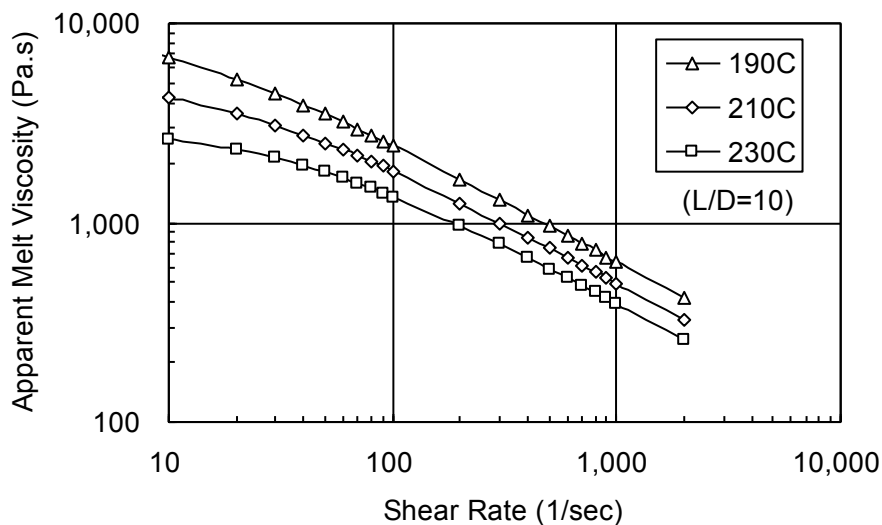
Fig. 1 Melt Viscosity of SoarnoL™ AT4403
